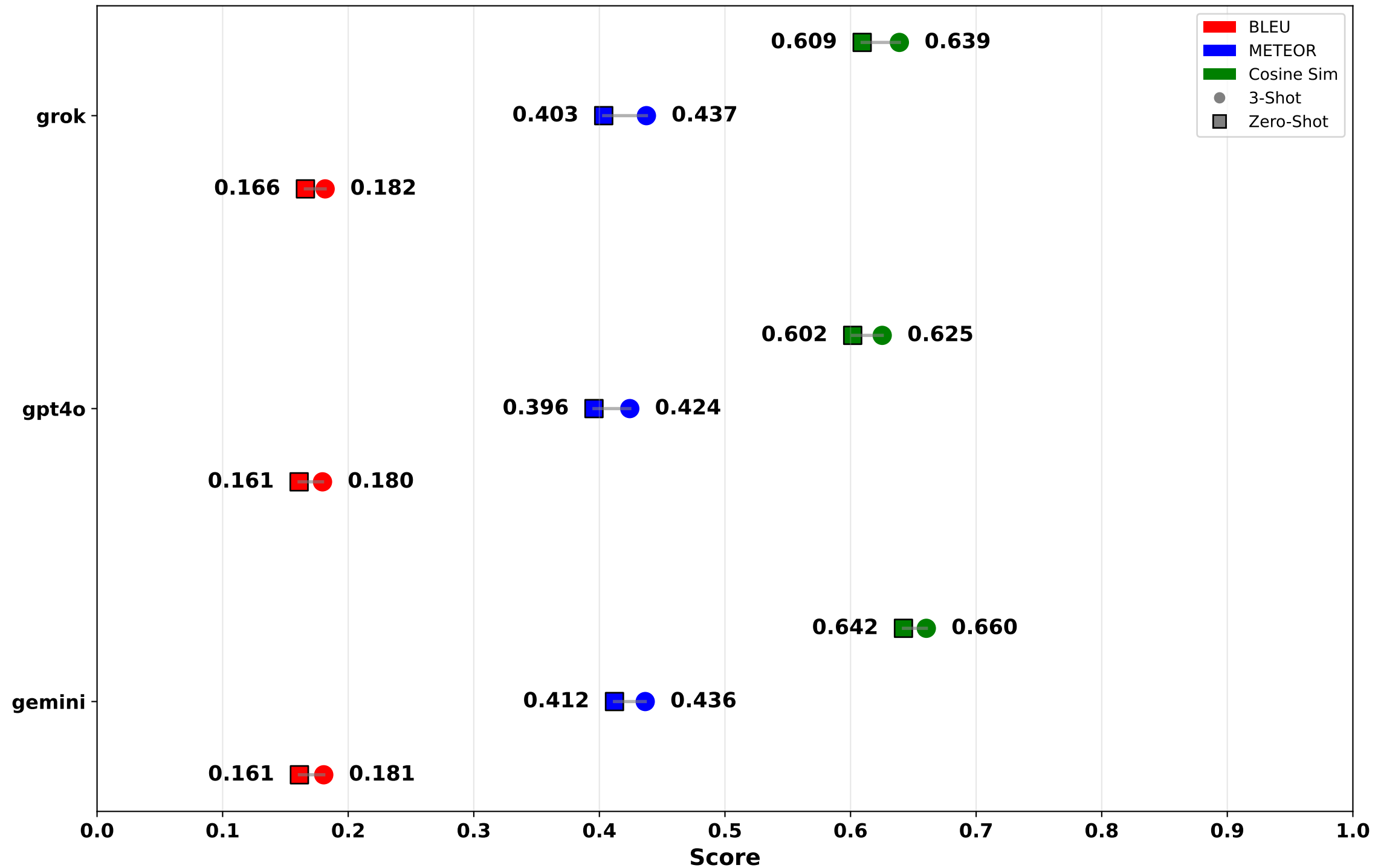
3-Shot vs Zero-Shot Performance
